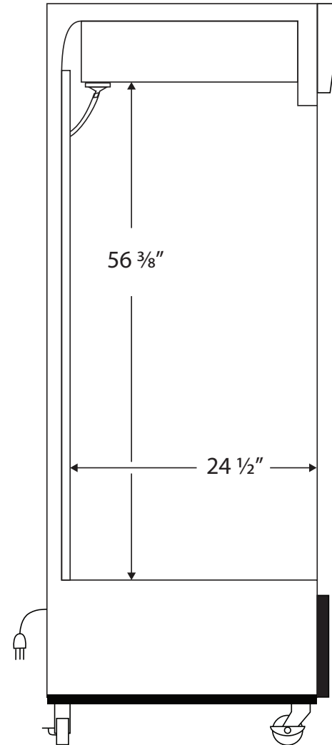
Side View
