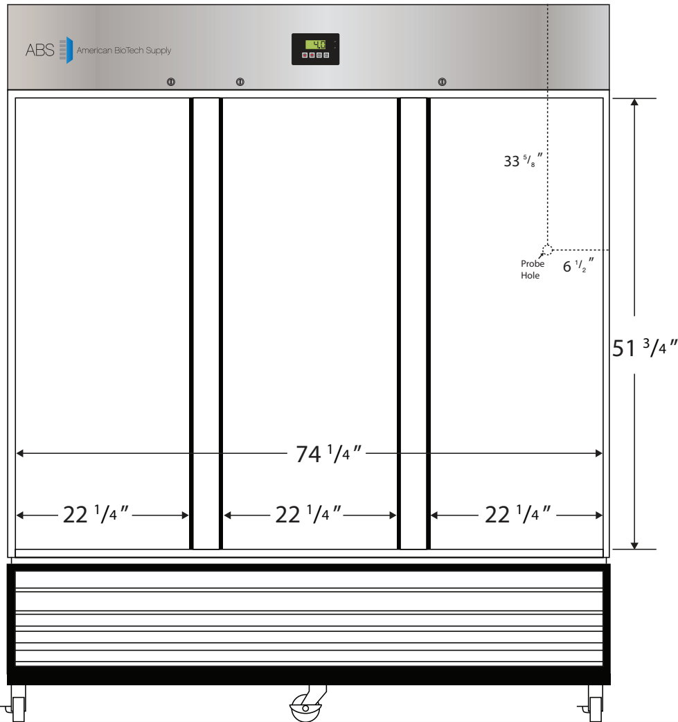
Front View
