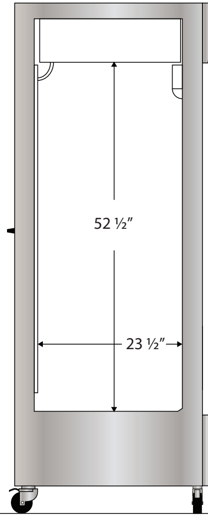
Side View
