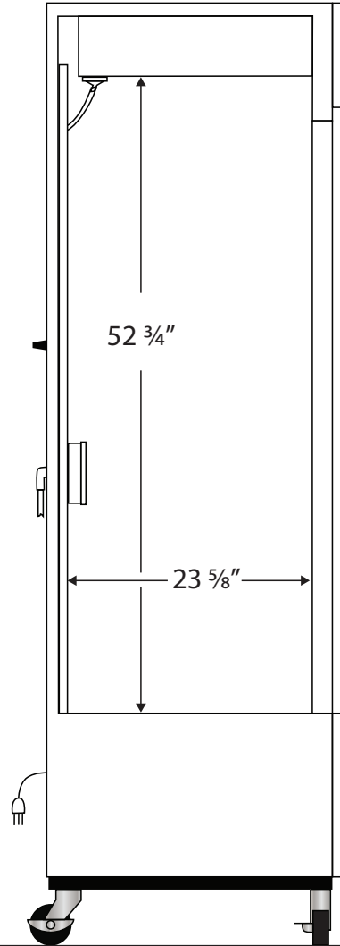
Side View
