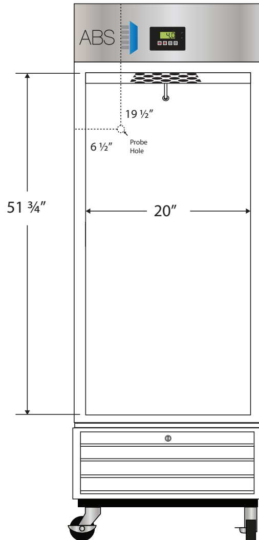
Front View
