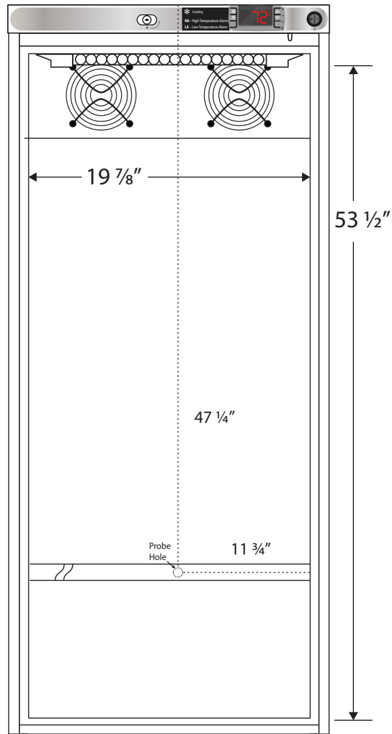
Front View
