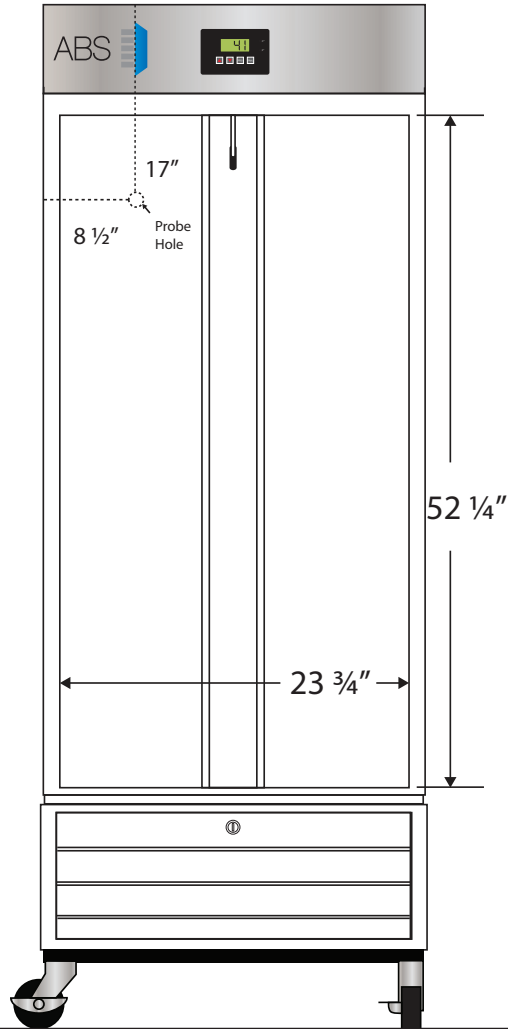
Front View
