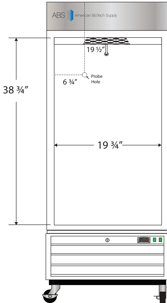
Front View
