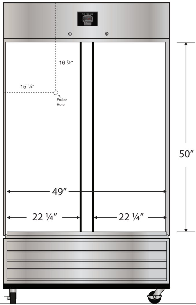
Front View
