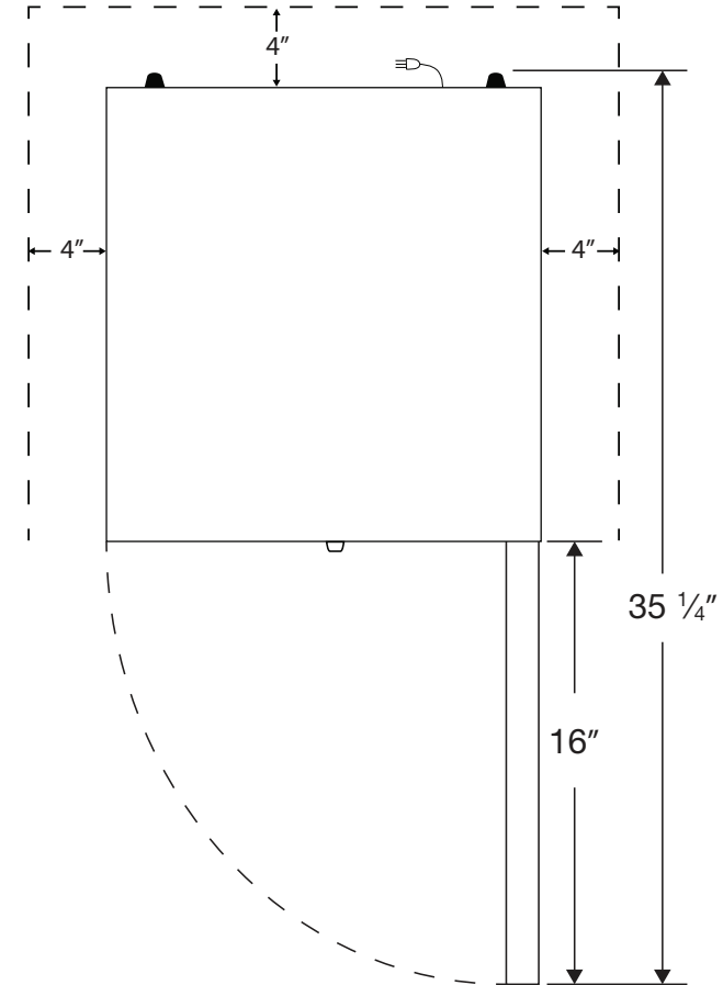
Top View
